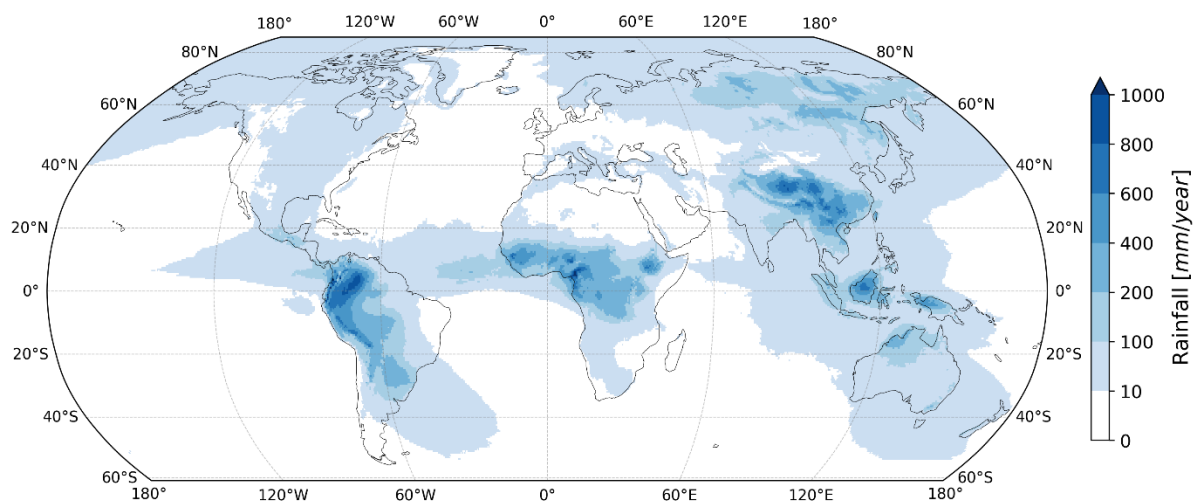
Figure 7: The global IPL evaporationshed spatial extent depicted with amount of precipitation (mm/year) contributed from IPL green water flow (average annual over the period 2007-2018).
