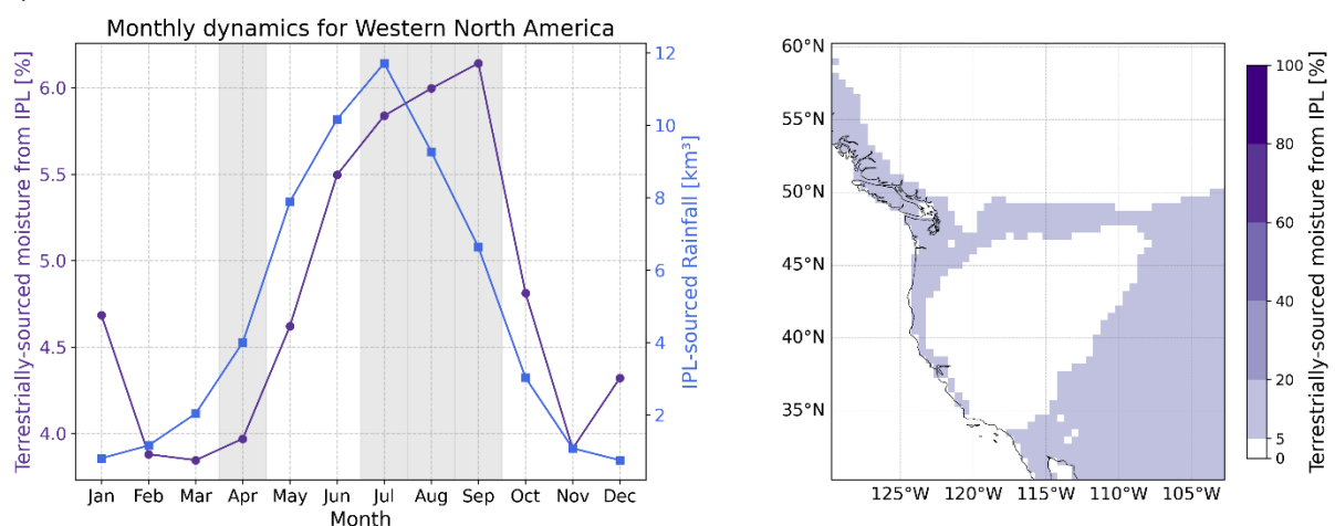
Figure 12: Regional analysis for each Giorgi region (a-u). The left panel shows the IPL sourced moisture per month both in terms of volume ( \text{km}^3 , blue line) and percentage of terrestrially sourced moisture (purple line). The dry season is indicated by the months shaded in grey. The right panel displays the proportion of terrestrially-sourced precipitation from IPL for each grid within the cropped Giorgi region.
